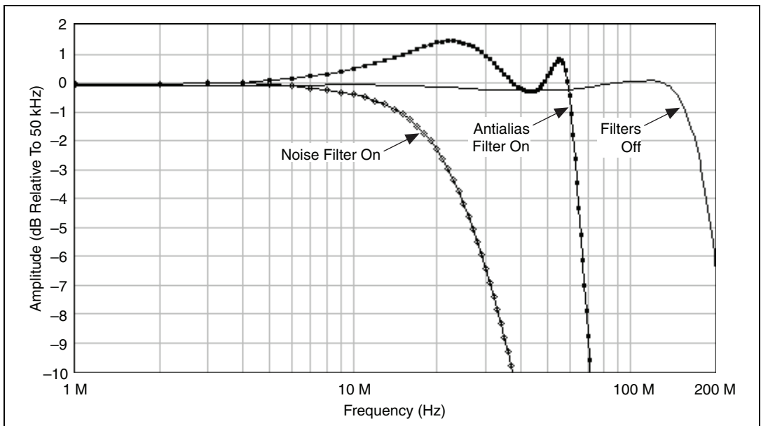
Figure 1. NI 5124 Frequency Response (Typical)
